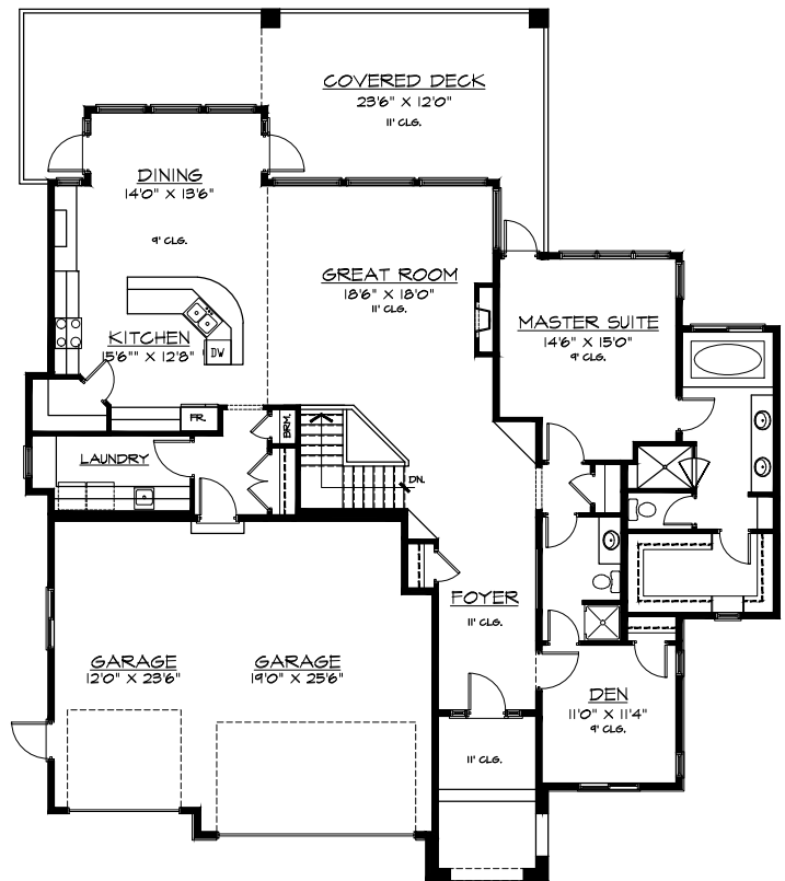
MAIN FLOOR PLAN 2081 SQ.FT.
