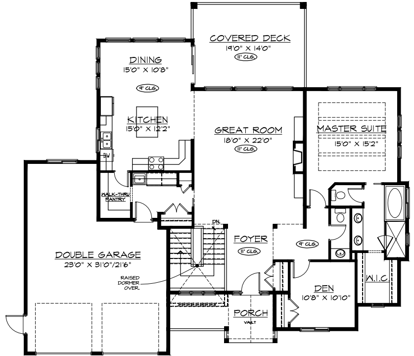
MAIN FLOOR PLAN 1808 SQ.FT.
