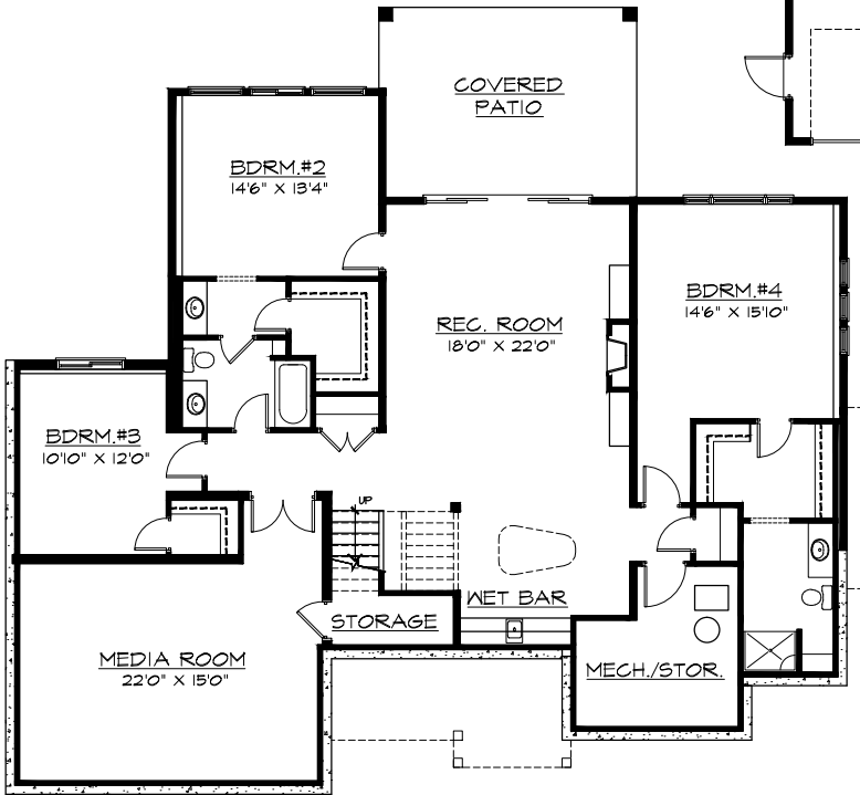
LOWER FLOOR PLAN 2147 SQ.FT. EXCLUDING STOR. & MECH.
