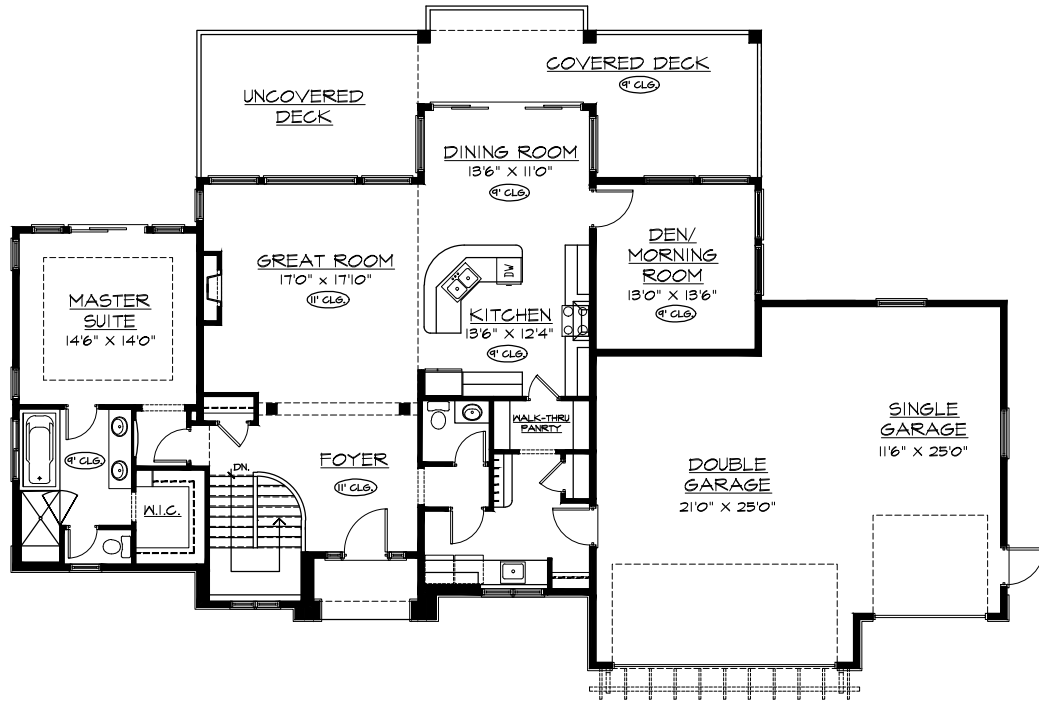
MAIN FLOOR PLAN 1792 SQ. FT.
