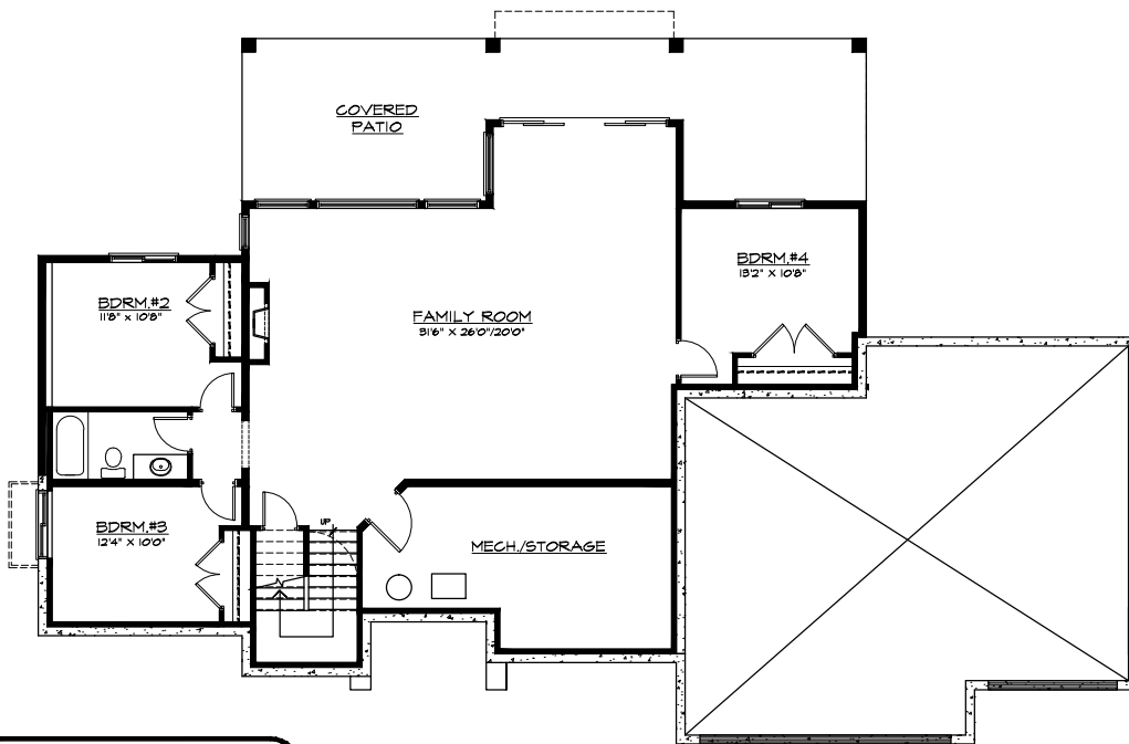
LOWER FLOOR PLAN 1377 SQ. FT.
