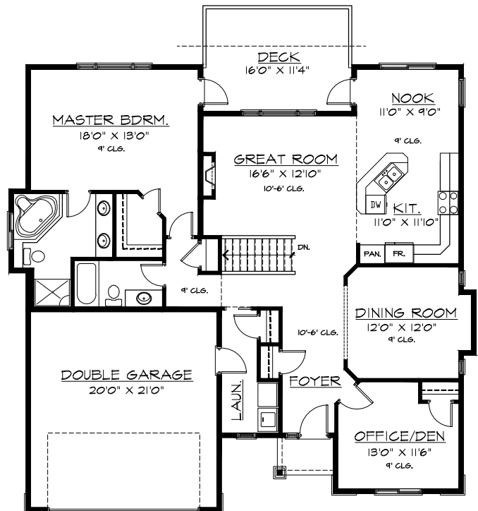
MAIN FLOOR PLAN 1633 SQ.FT.
