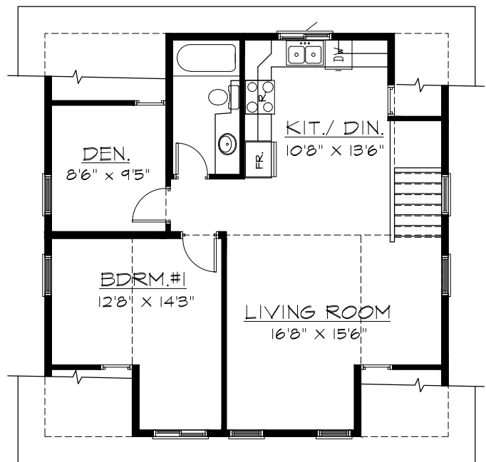
UPPER FLOOR PLAN 757 SQ.FT.
