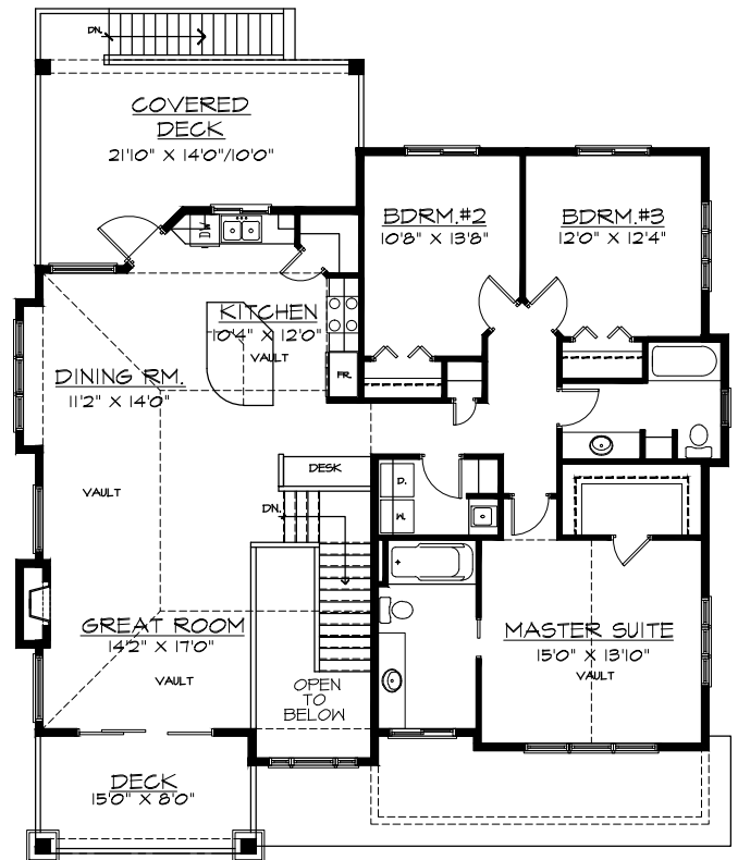
MAIN FLOOR PLAN 1637 SQ.FT.
