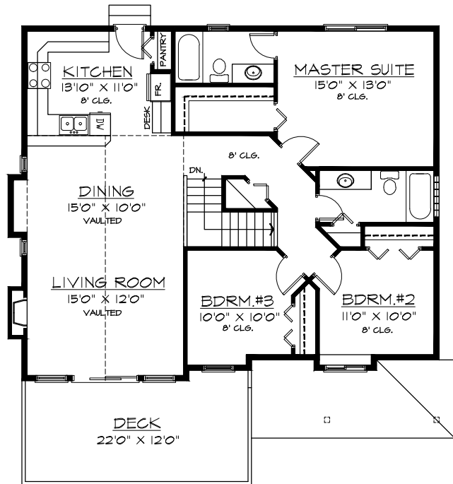
MAIN FLOOR PLAN 1326 SQ.FT.
