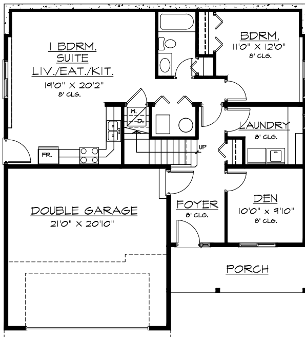
LOWER FLOOR PLAN FOYER/DEN/LAUNDRY 322 SQ. FT. ONE BDRM. SUITE 673 SQ. FT.
