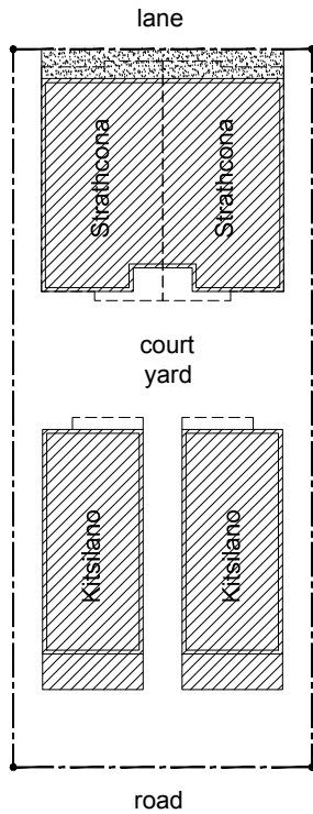
Inhabit Residential RU7 Typical Site Layout
