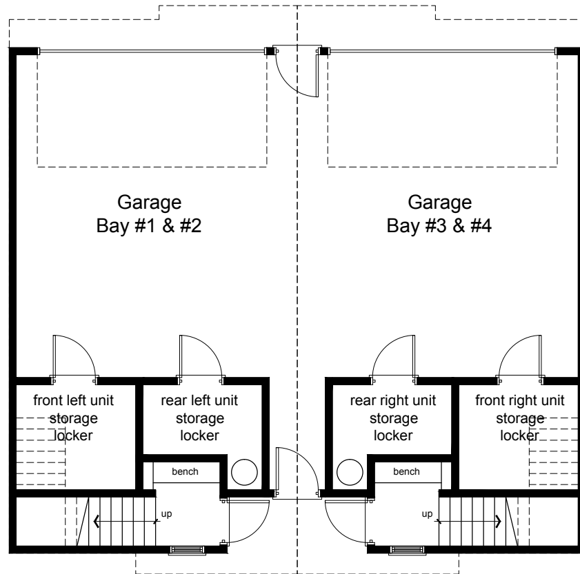
First Floor - Garage Plan Foyer 43 sq.ft. / unit
