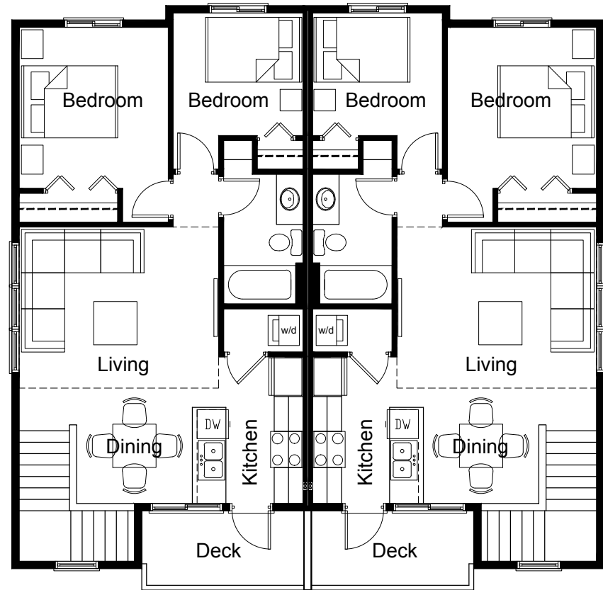
Second Floor - Main Floor Plan 743 sq.ft. / unit
