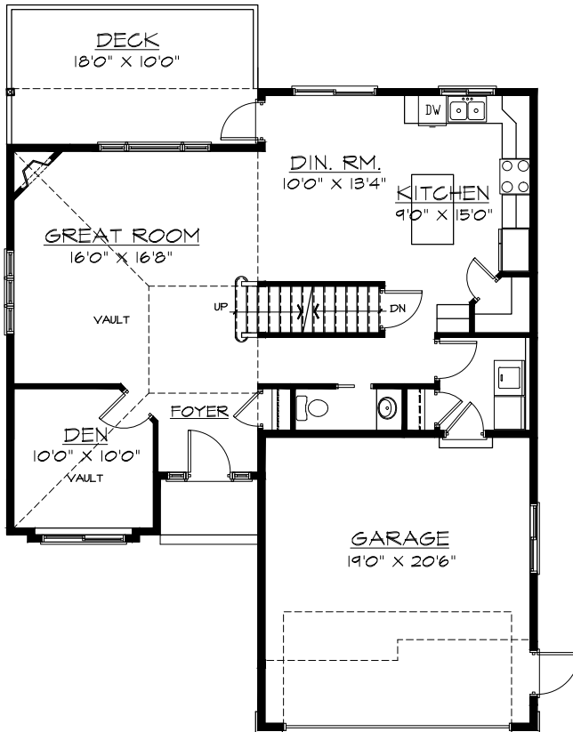
MAIN FLOOR PLAN 981 SQ.FT.
