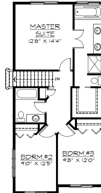
UPPER FLOOR PLAN 791 SQ.FT.
