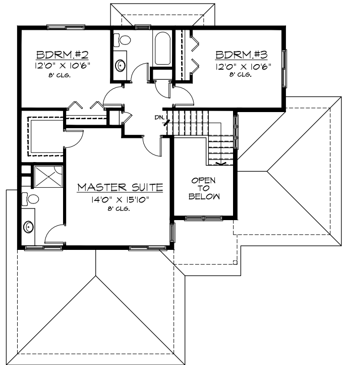
UPPER FLOOR PLAN 798 SQ.FT.
