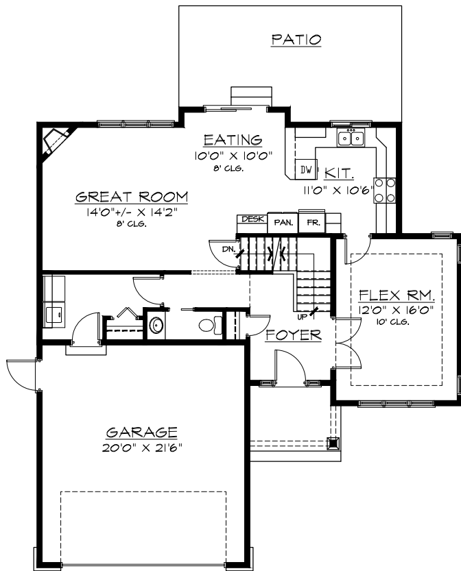
MAIN FLOOR PLAN 987 SQ.FT.
