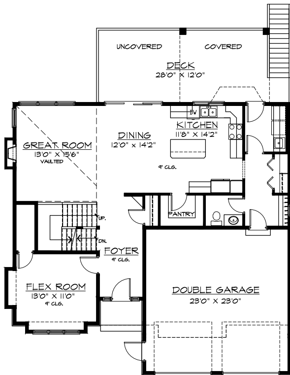
MAIN FLOOR PLAN 1248 SQ.FT.
