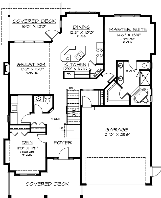
MAIN FLOOR PLAN 1559 SQ.FT.
