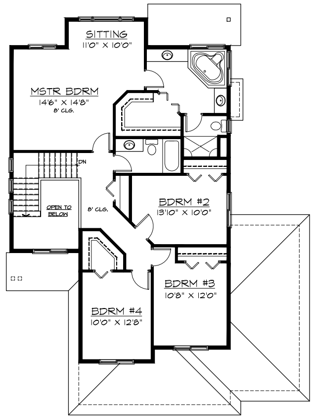
UPPER FLOOR PLAN 1194 SQ.FT.
