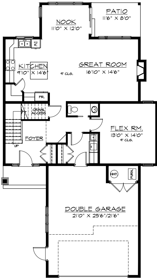
MAIN FLOOR PLAN 1116 SQ.FT.
